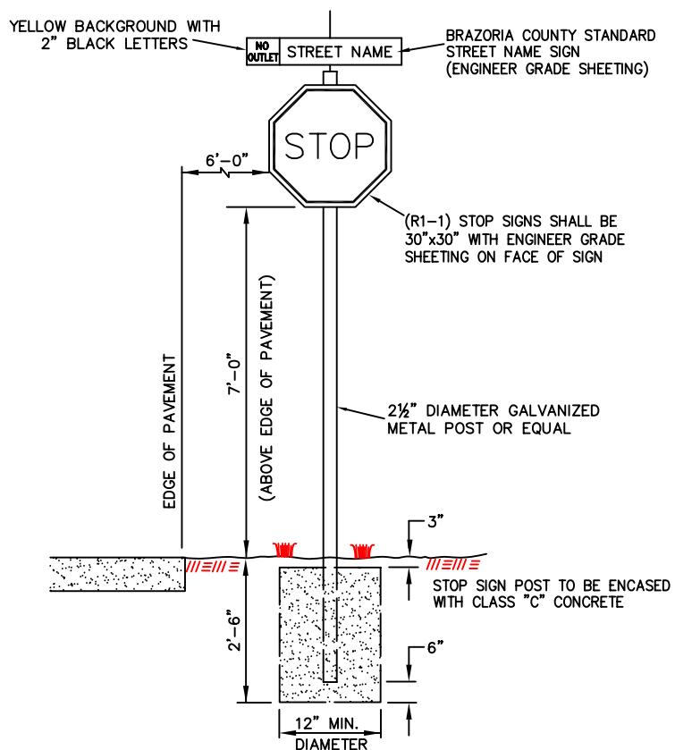
SIGN MOUNT
